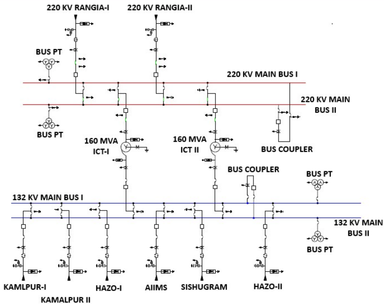
SLD OF 220/132 KV AMINGAON GIS
